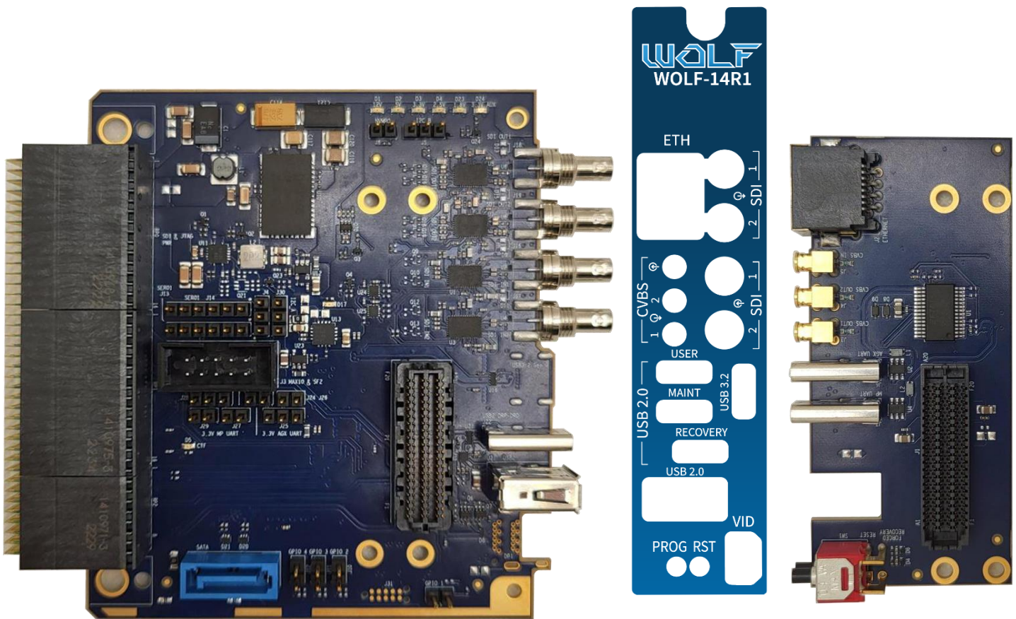
The WOLF 14R1 consists of a Main board and a daughter board
